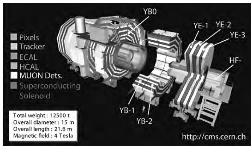
Figure 5: The Compact Muon Solenoid detector with its major components: the magnet, the tracking detector, the calorimeters and the muon system.
