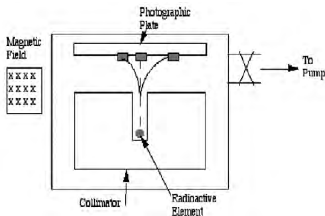
Figure 2: Schematic diagram of Becquerel's experiment and emulsion picture for the discovery of pions.
