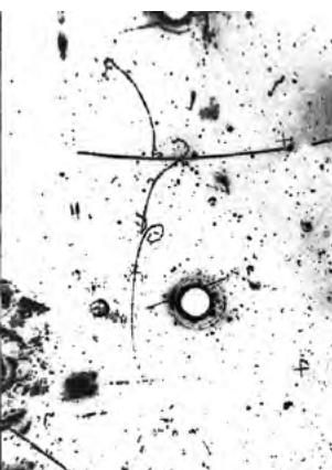
Figure 4: Picture of the Gargamelle bubble chamber and one of the neutral current candidates as observed in this experiment.
