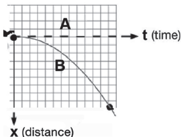
Figure 1: The space-time diagram for a ball released at waist high.
